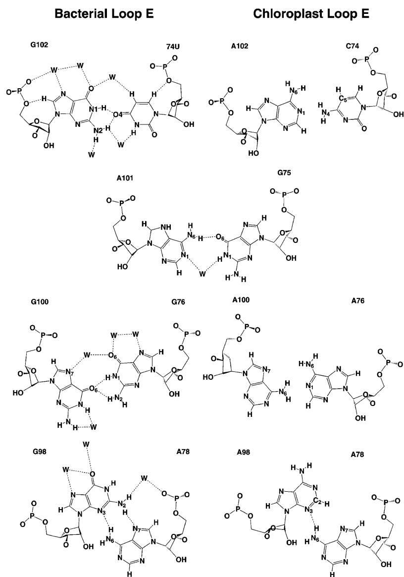
FIGURE 2 Structures of corresponding non-Watson-Crick basepairs in the bacterial Loop E and in spinach chloroplast Loop E. The bacterial basepairs ( left ) are taken from the high-resolution crystal structure (NDB file URL064) whereas the corresponding chloroplast basepairs are shown as initially modeled based on isosteric considerations (Leontis and Westhof, 1998b). ( Top ) Cis bifurcated G/U and A/C. Middle two rows: Water-inserted cis Watson-Crick G/A followed by cis bifurcated G/G and A/A. ( Bottom ) trans Hoogsteen/Sugar-edge (sheared) G/A and A/A.
